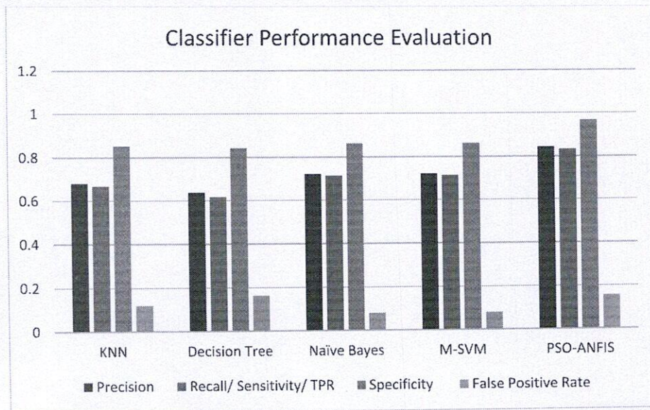
Fig. 6. Performance evaluation of different classifiers
