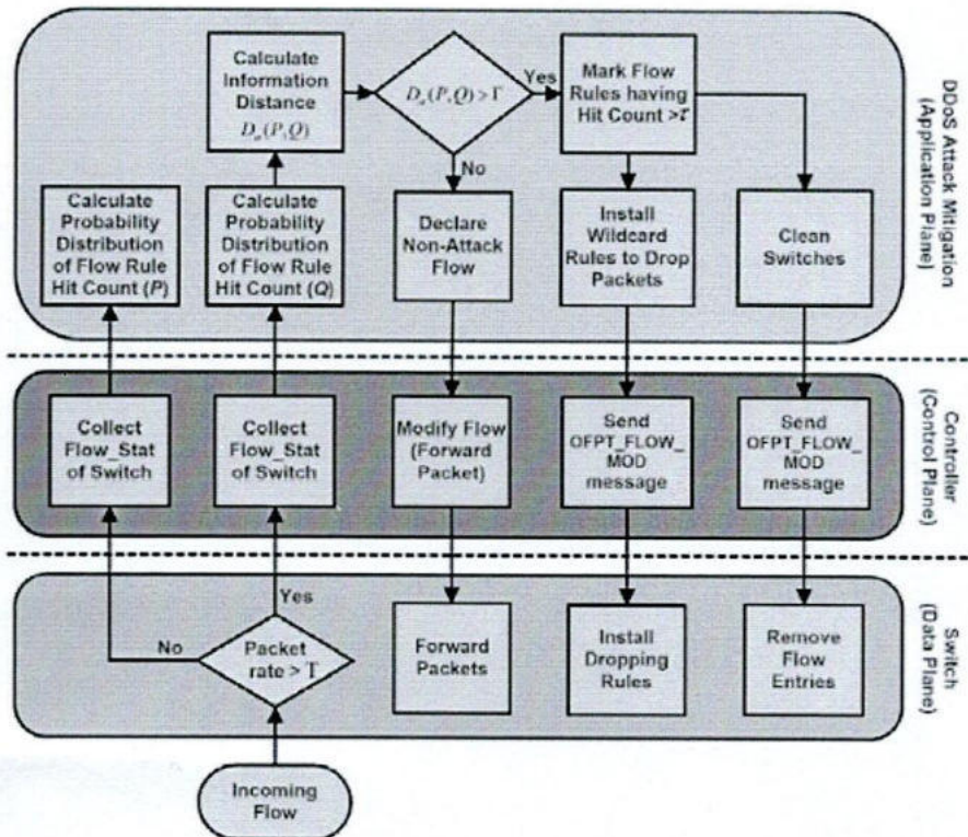
Figure 2. SDN based DDoS attack model
