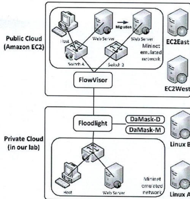
Figure 3 Cloud and SDN based DDoS attack model
