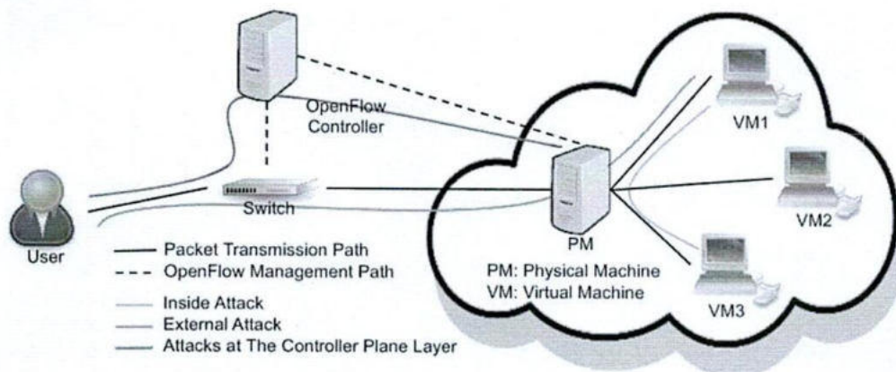
Figure 4 Dynamic entropy based attack model
