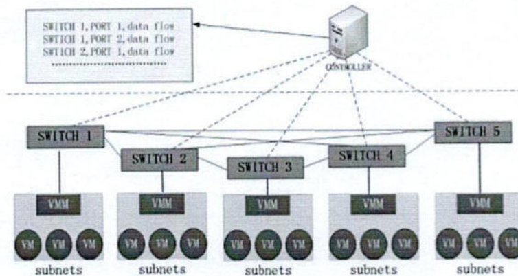
Figure 1 SVM based DDoS attack Model
